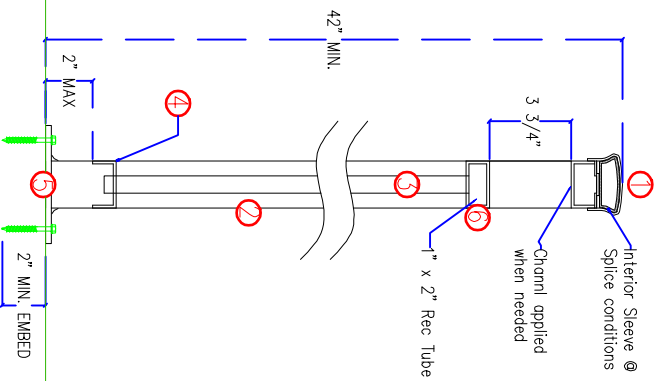
Typical Open Three Rail Detail
