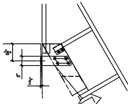
MODEL 335 BRACKET MAT'L: 3/8" ALUM 6061-T6
